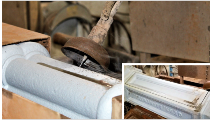
Own water jet robot system
